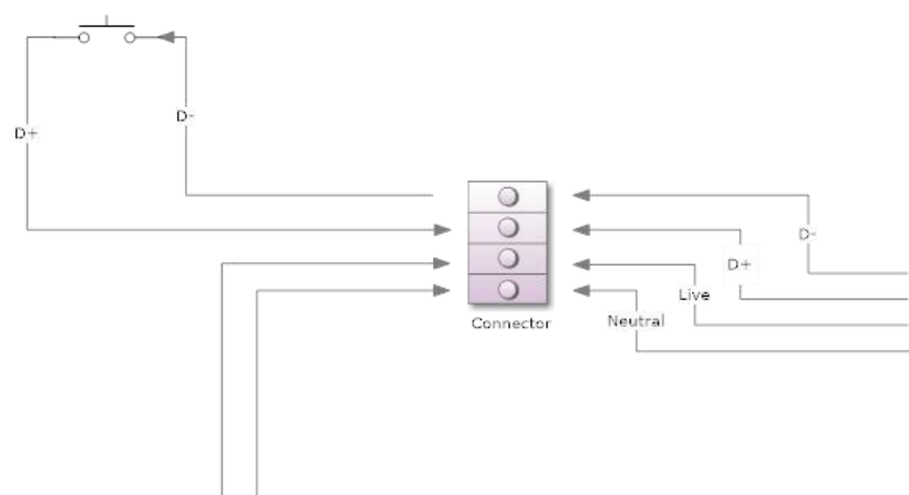
Momentary Switch (Switch DIM)
