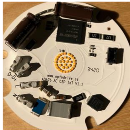
LED Module with IoT (DimIn Switch)
