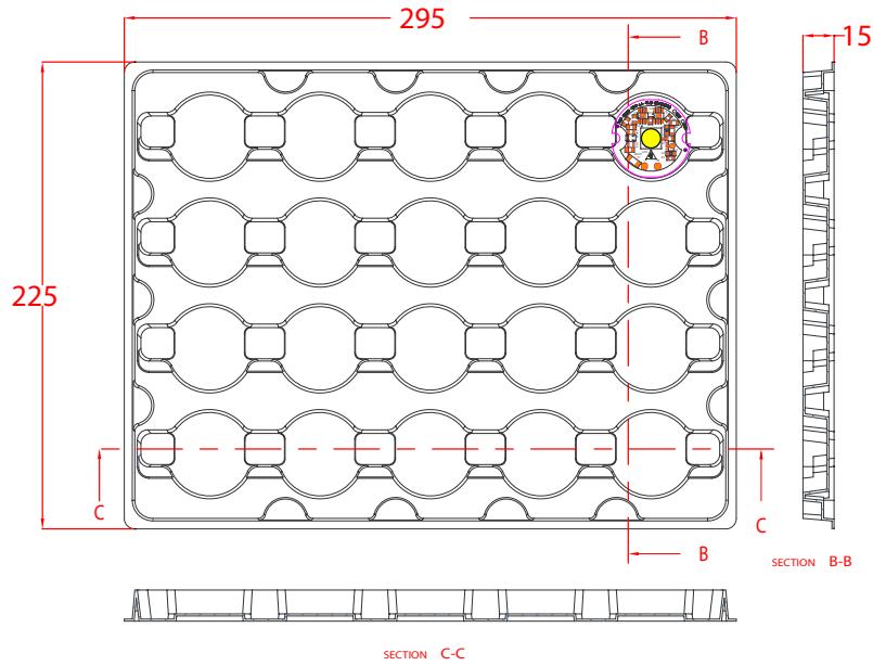
Tray : 295x225x15 mm ,20pcs Module In the Tray
