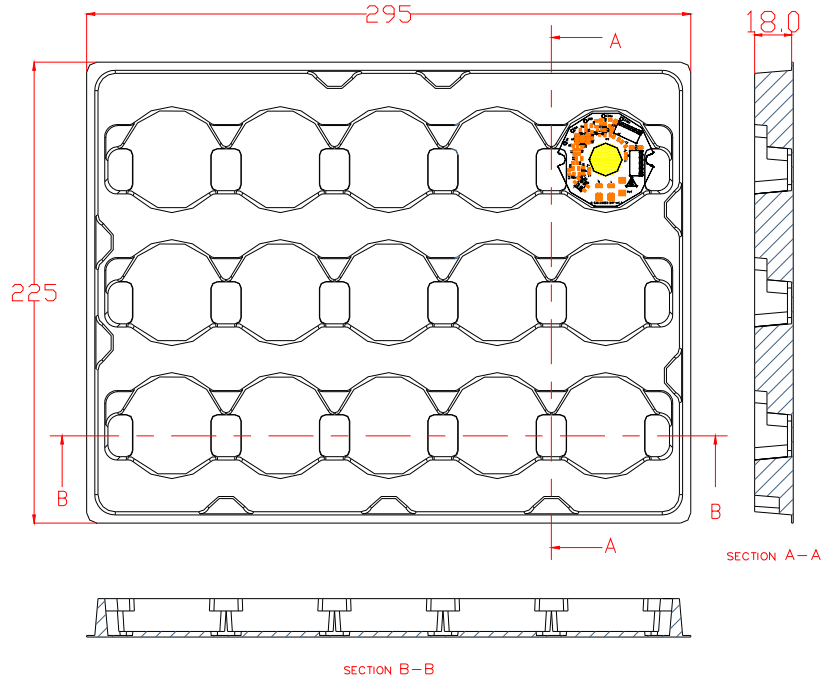
Tray:295x225x18mm, 15pcs module in the Tray
