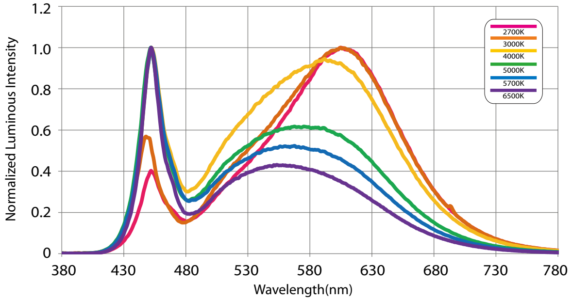
Color Spectrum(Tc=25°C,VAC=230V)_Ra 80
