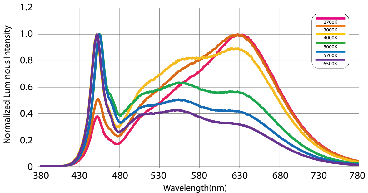
Color Spectrum(Tc=25°C,VAC=230V)_Ra 90
